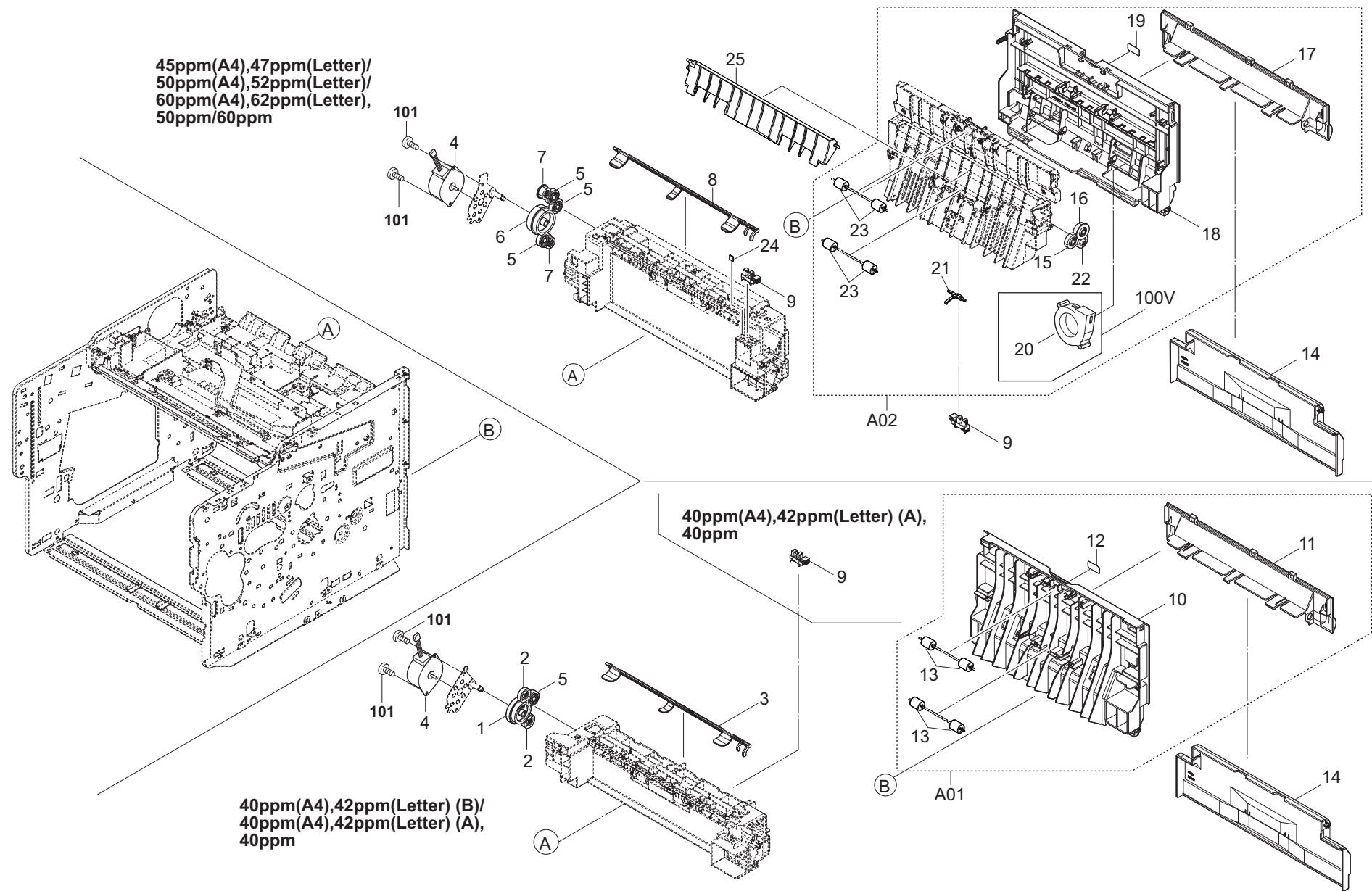
FIG. 8 Exit Section
