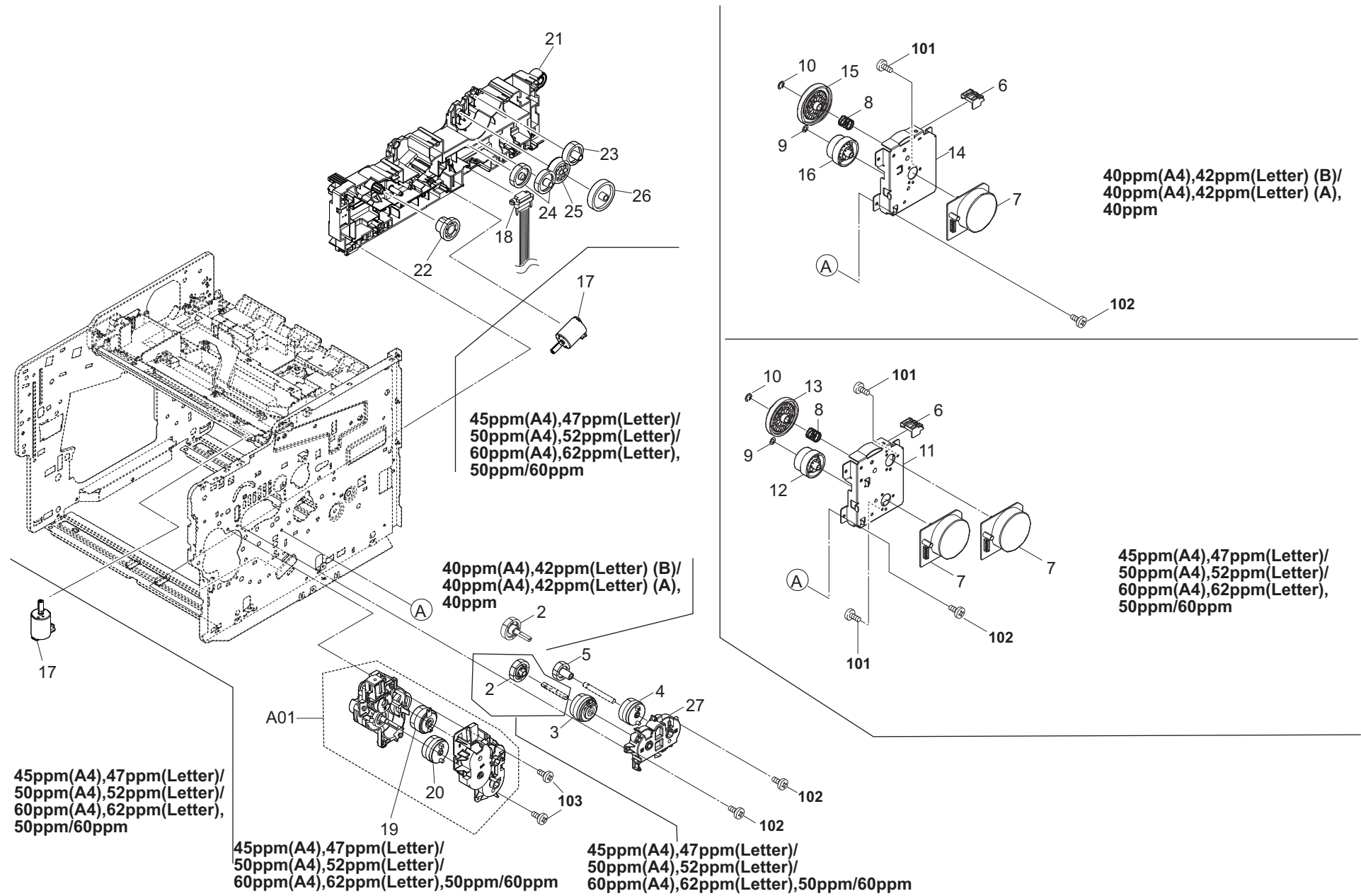
FIG. 9 Drive Section
