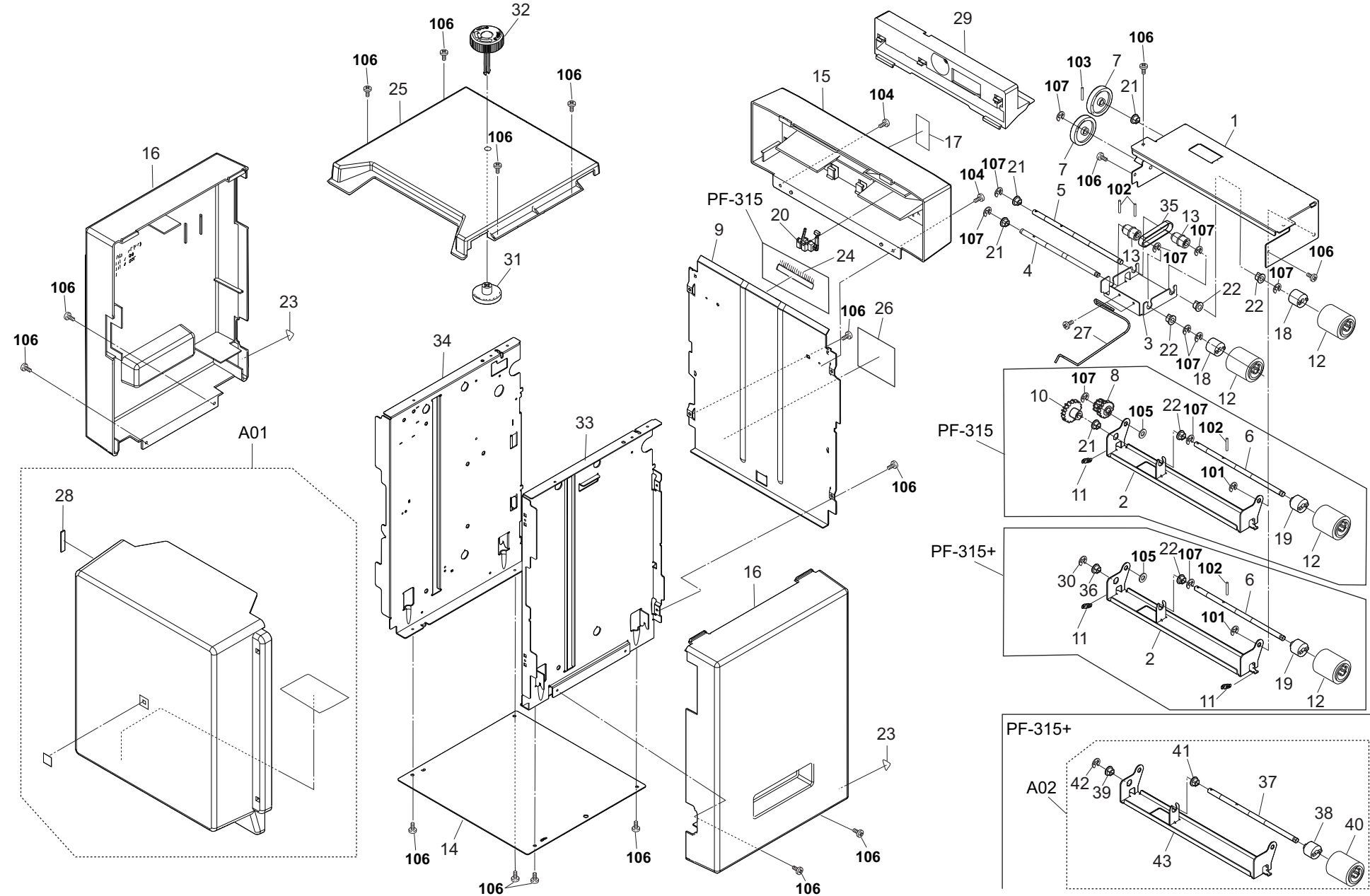
FIG. 1 Bulk Paper Feeder 1
