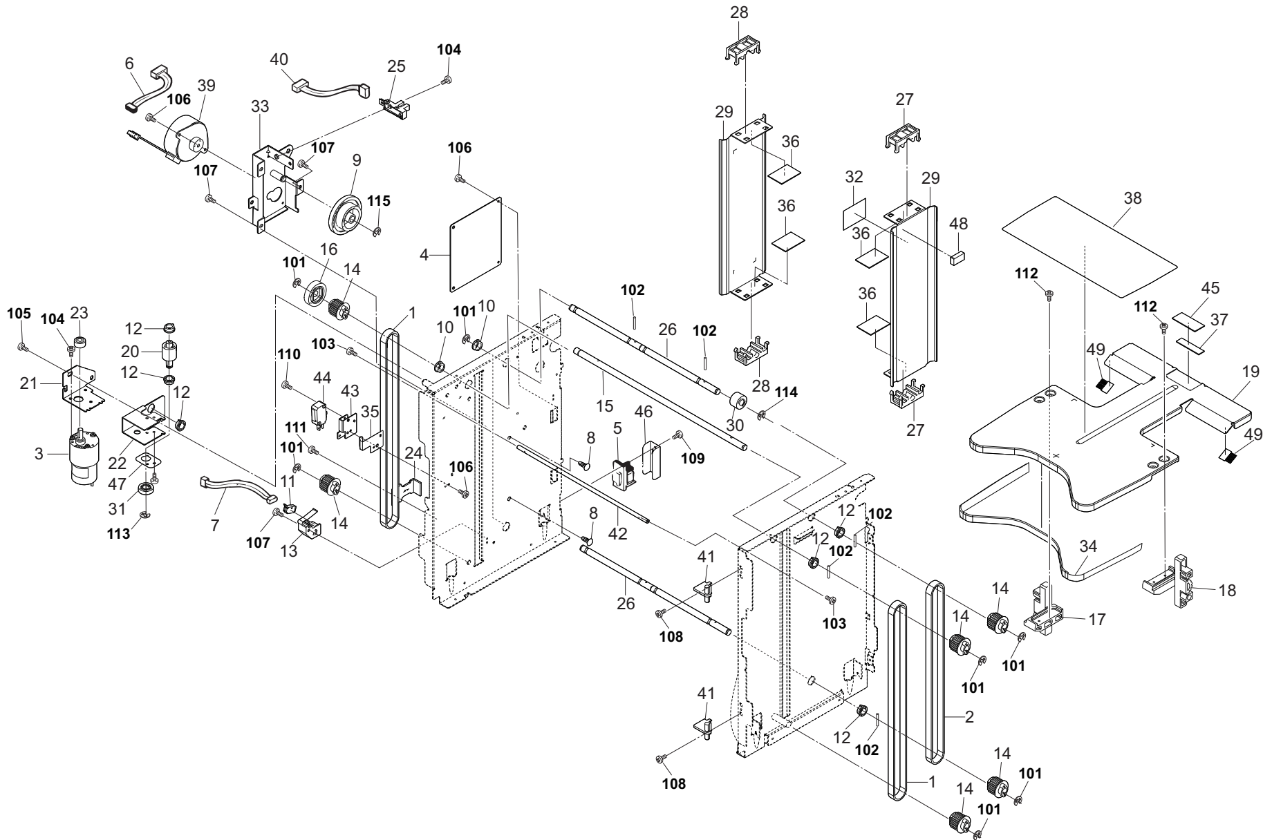
FIG. 2 Bulk Paper Feeder 2
