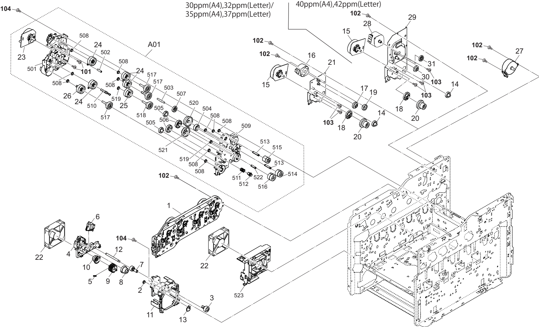
FIG. 12 Drive Section
