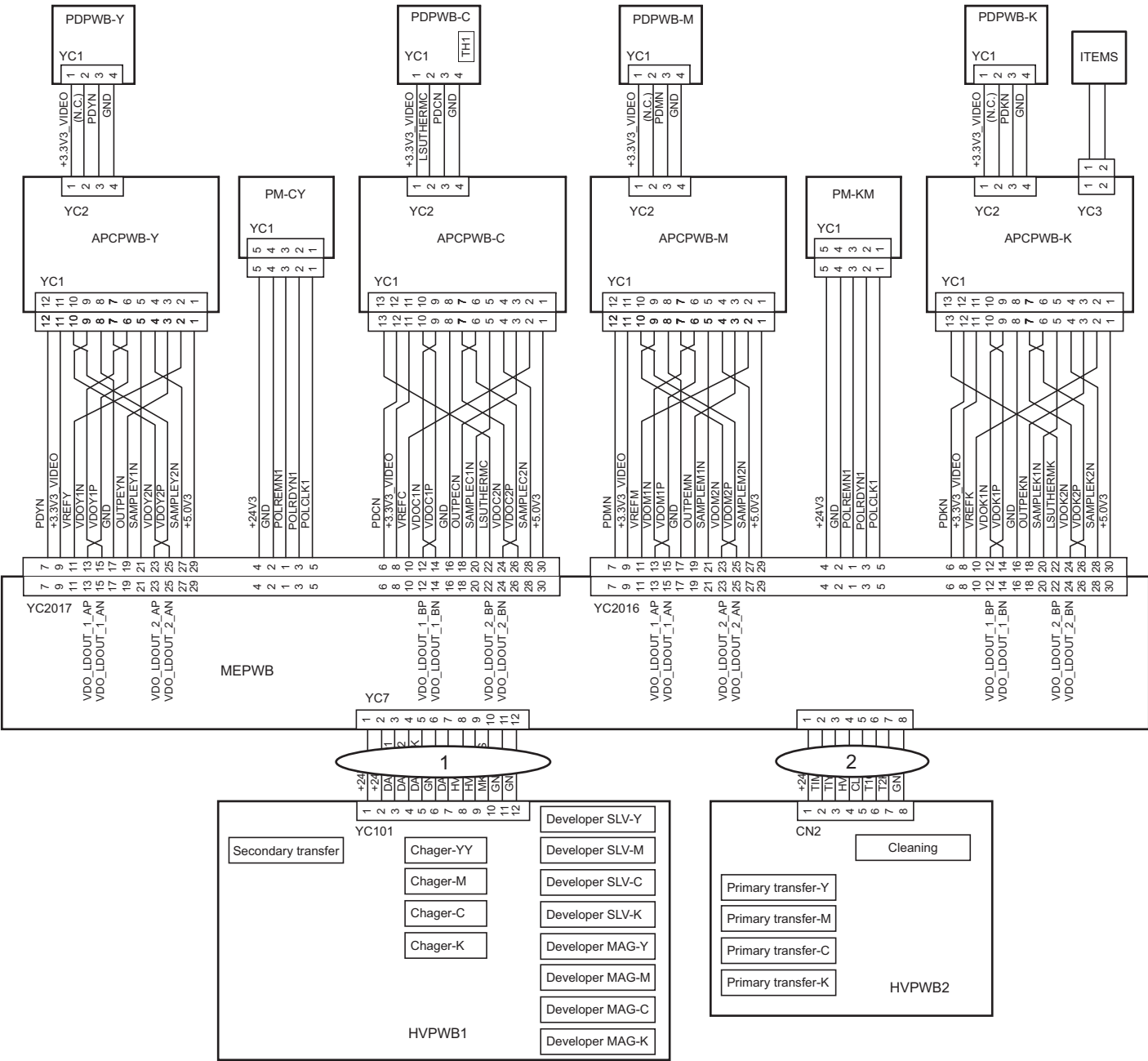
FIG. 17 Wire Section 2 (40ppm(A4),42ppm(Letter))
